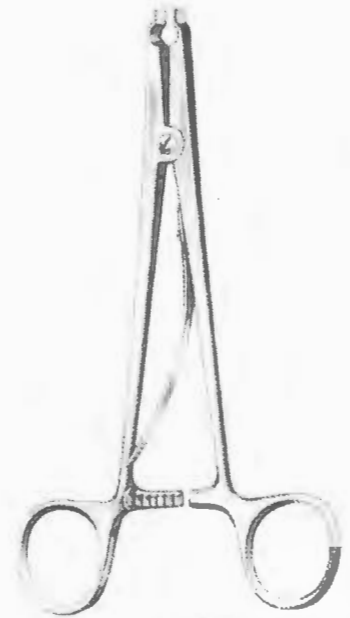
-10S-056 Raney Hemostatic Clip Applying Forceps 6" (15 cm)
